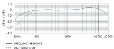
Frequency response
